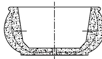
4 CROSS SECTION
