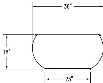
2 ELEVATION VIEW
