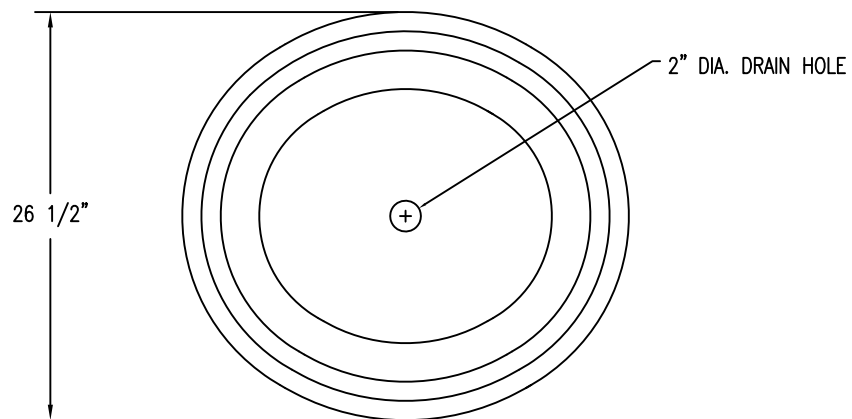
1 TOP VIEW
