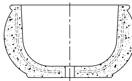
4 CROSS SECTION
