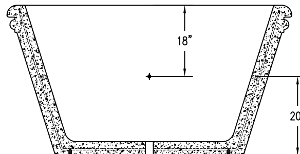
4 CROSS SECTION
