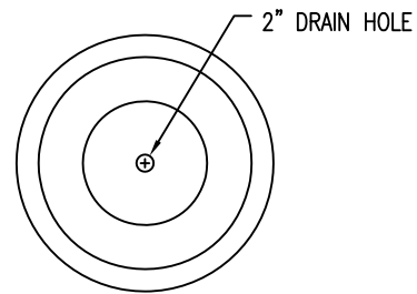
1 TOP VIEW
