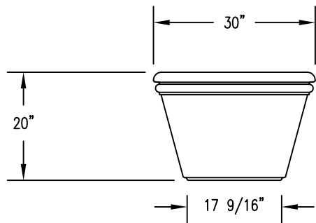
2 ELEVATION VIEW
