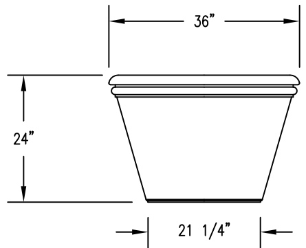
2 ELEVATION VIEW
