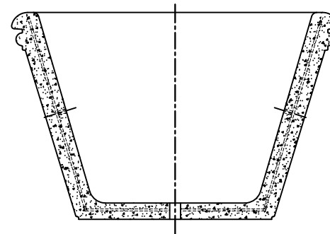
4 CROSS SECTION
