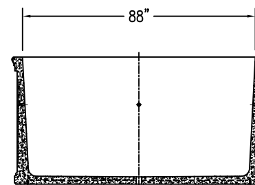
4 CROSS SECTION
