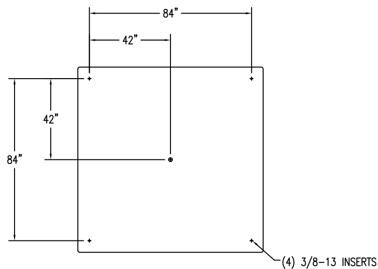
3 BOTTOM VIEW
