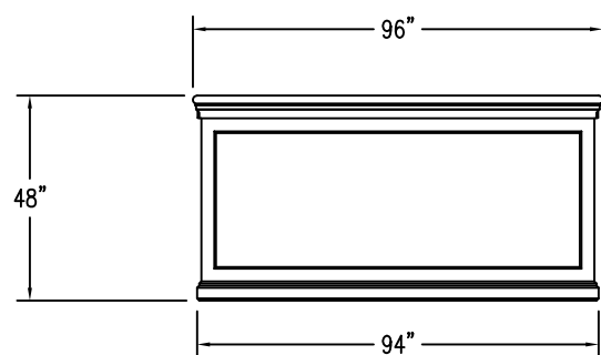
2 ELEVATION VIEW
