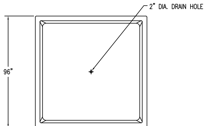
1 TOP VIEW
