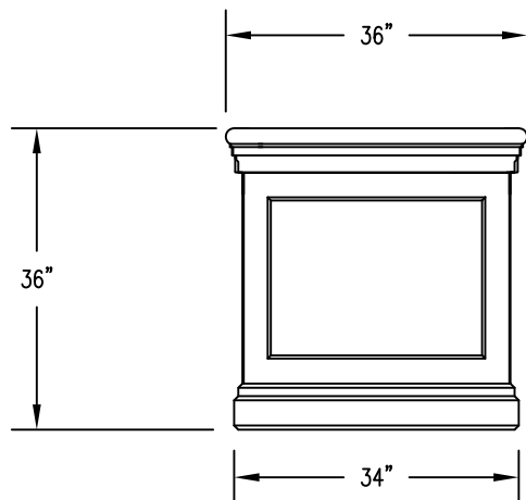
2 ELEVATION VIEW
