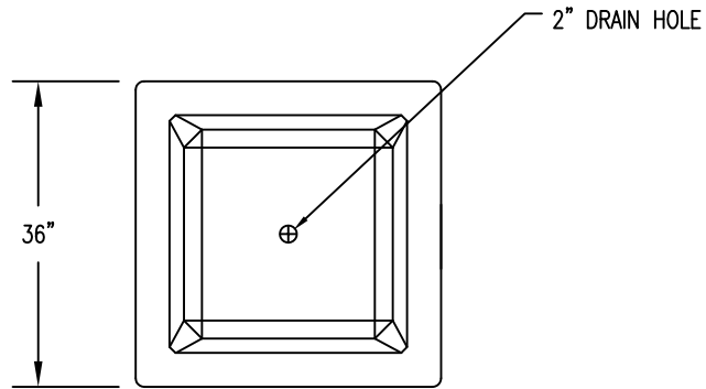
1 TOP VIEW
