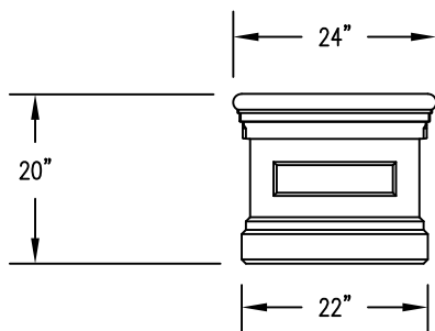
2 ELEVATION VIEW
