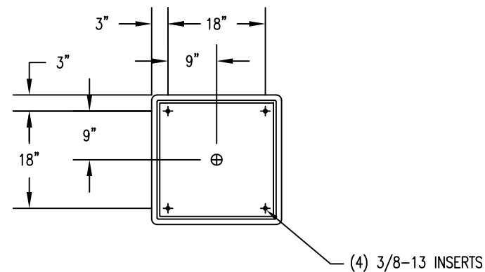
3 BOTTOM VIEW
