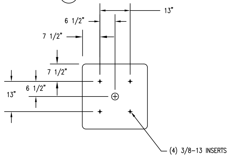
3 BOTTOM VIEW
