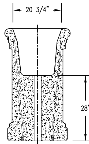
4 CROSS SECTION
