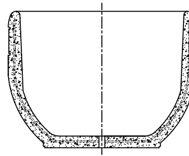
4 CROSS SECTION
