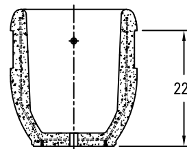
4 CROSS SECTION
