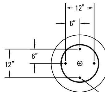
3 BOTTOM VIEW (4) 1/2-13 INSERTS
