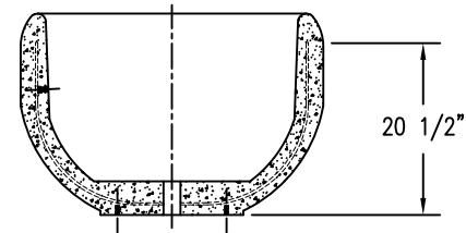
4 CROSS SECTION
