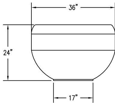
2 ELEVATION VIEW
