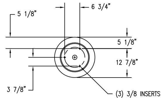
3 BOTTOM VIEW
