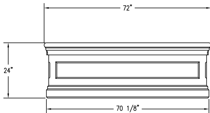
2 ELEVATION VIEW
