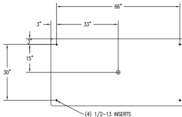
3 BOTTOM VIEW
