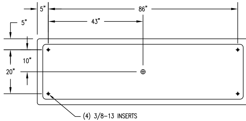
3 BOTTOM VIEW
