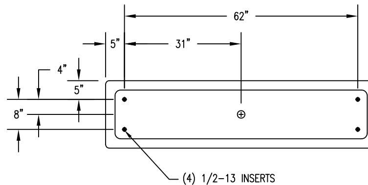
3 BOTTOM VIEW
