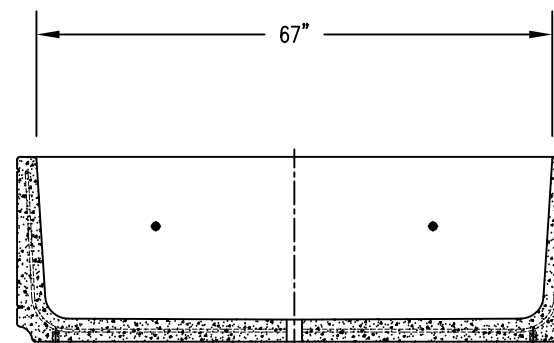
4 CROSS SECTION
