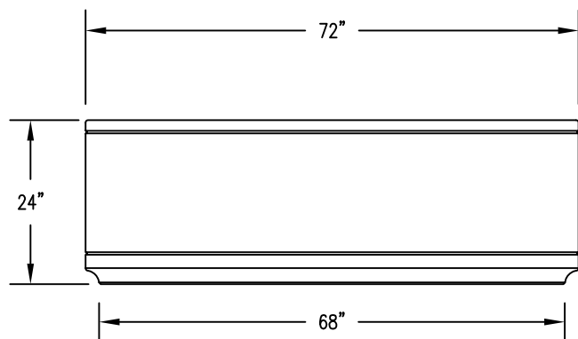
2 ELEVATION VIEW
