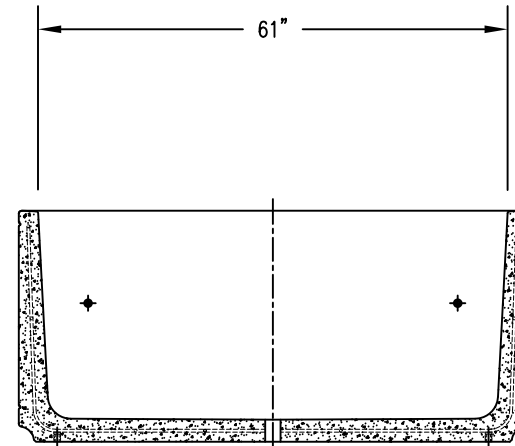
4 CROSS SECTION
