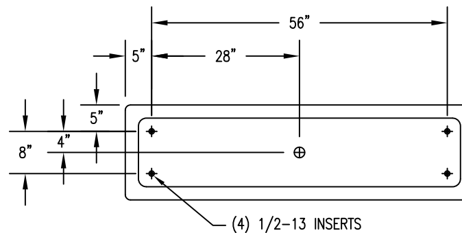
3 BOTTOM VIEW
