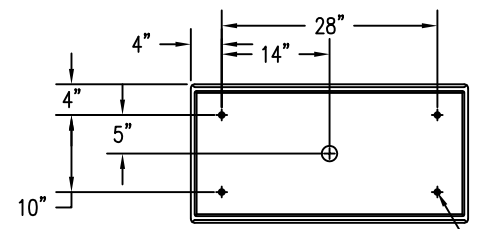
3 BOTTOM VIEW
