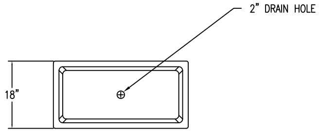
1 TOP VIEW
