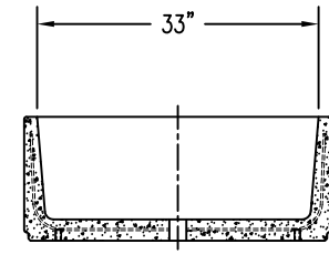
4 CROSS SECTION
