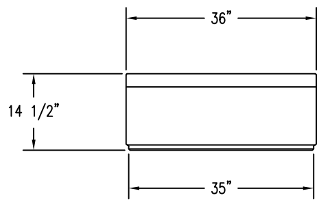
2 ELEVATION VIEW
