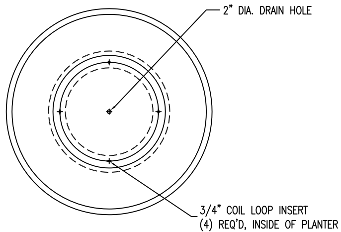
1 TOP VIEW
