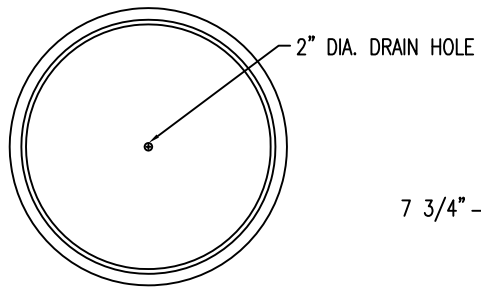
1 TOP VIEW
