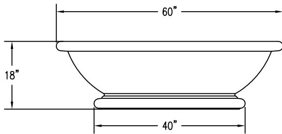
2 ELEVATION VIEW
