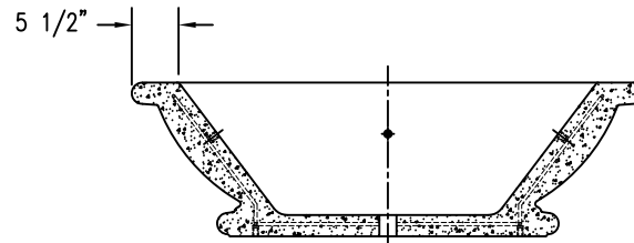
4 CROSS SECTION
