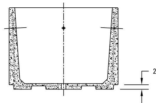
4 CROSS SECTION
