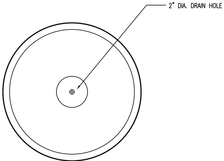
1 TOP VIEW
