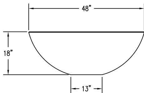
2 ELEVATION VIEW
