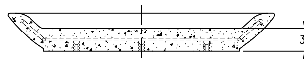
4 CROSS SECTION
