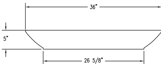
2 ELEVATION VIEW
