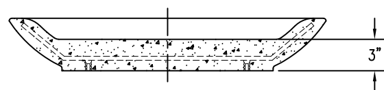
4 CROSS SECTION
