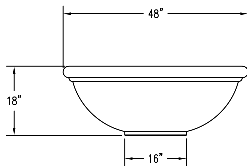
2 ELEVATION VIEW
