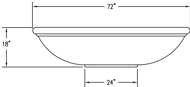
2 ELEVATION VIEW
