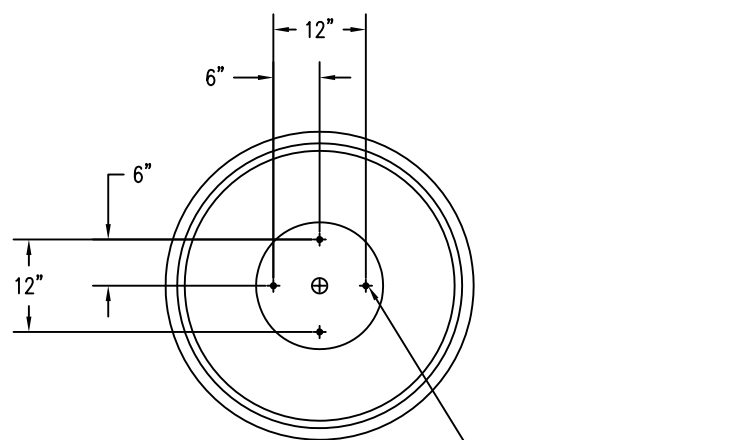
3 BOTTOM VIEW
