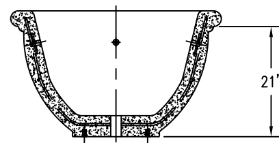
4 CROSS SECTION
