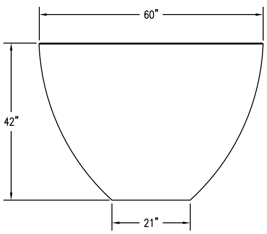
2 ELEVATION VIEW
