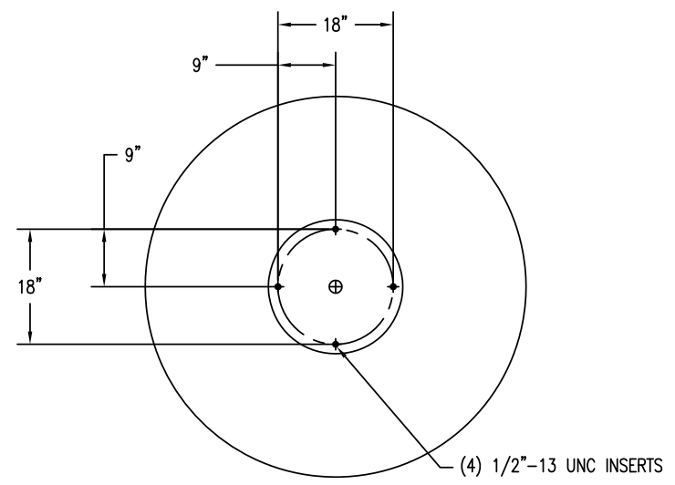
3 BOTTOM VIEW
