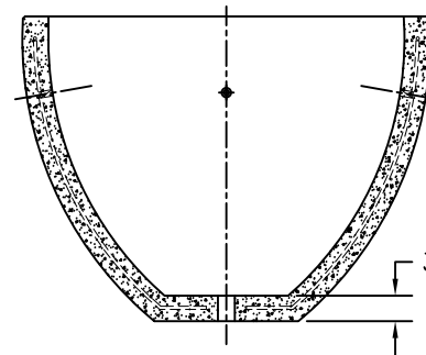
4 CROSS SECTION
