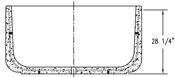
4 CROSS SECTION
