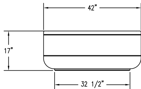
2 ELEVATION VIEW
