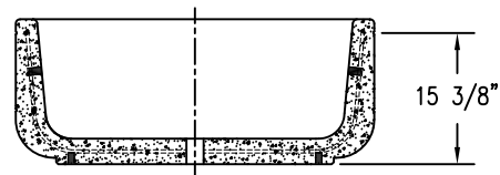
4 CROSS SECTION
