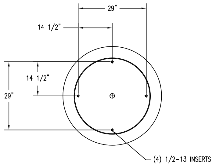
3 BOTTOM VIEW
