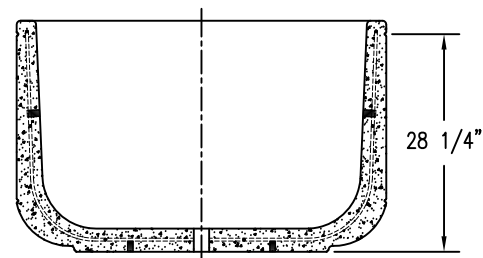
4 CROSS SECTION
