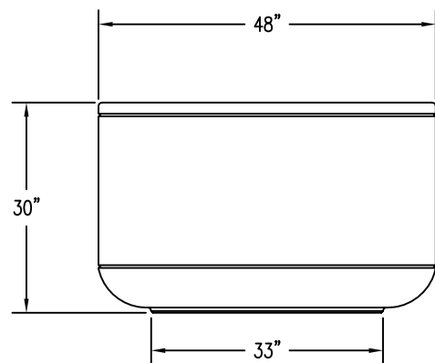
2 ELEVATION VIEW
