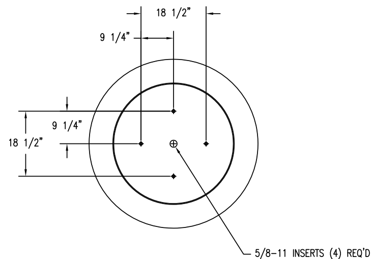
3 BOTTOM VIEW
