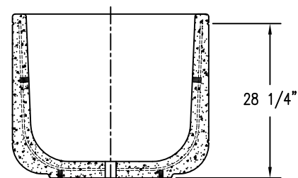
4 CROSS SECTION
