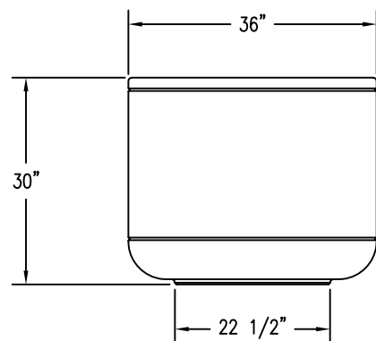
2 ELEVATION VIEW
