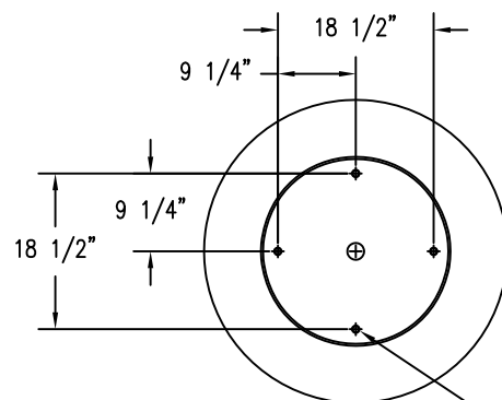
3 BOTTOM VIEW
