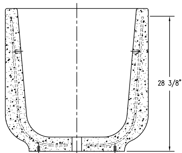
4 CROSS SECTION
