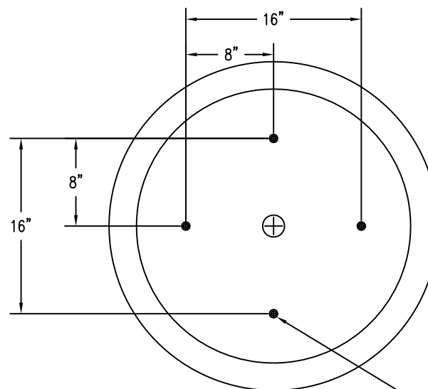
3 BOTTOM VIEW
