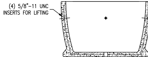
4 CROSS SECTION
