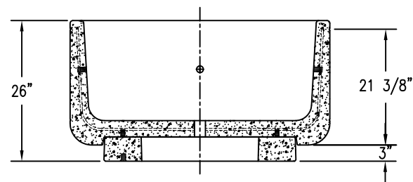
4 CROSS SECTION
