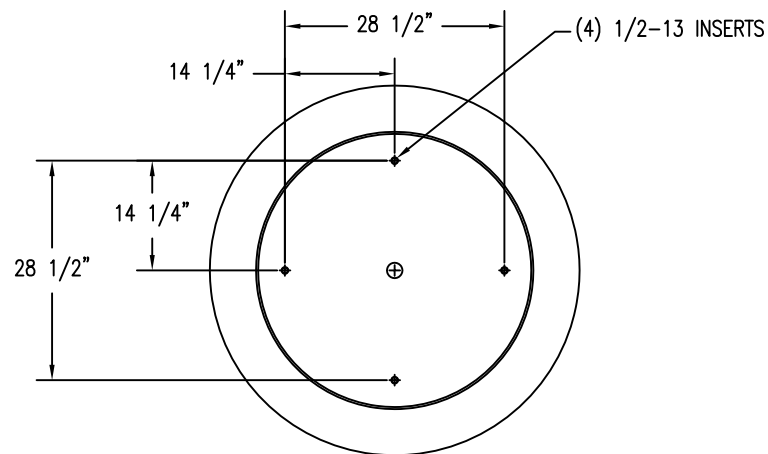
3 BOTTOM VIEW
