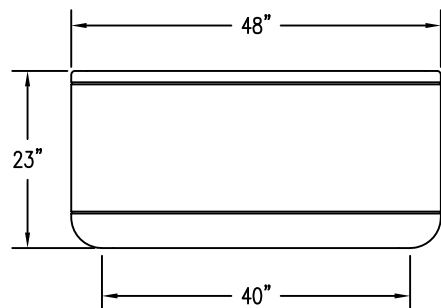
2 ELEVATION VIEW
