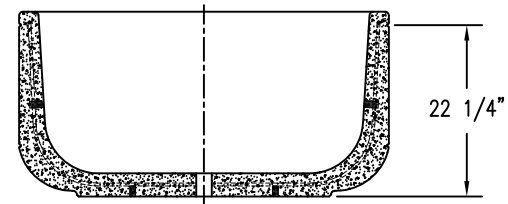
4 CROSS SECTION
