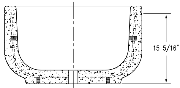
4 CROSS SECTION
