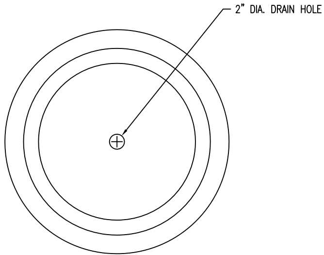
1 TOP VIEW
