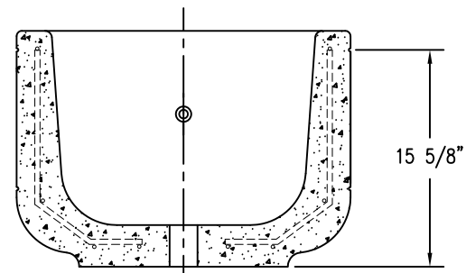
4 CROSS SECTION
