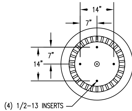
4 CROSS SECTION
