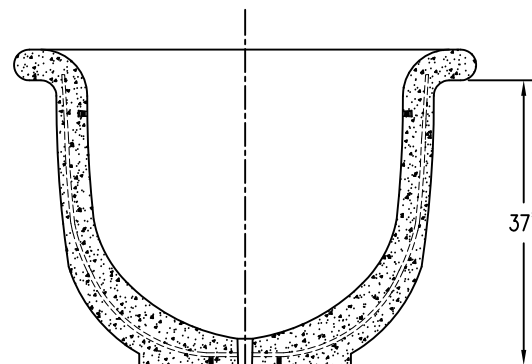
4 CROSS SECTION
