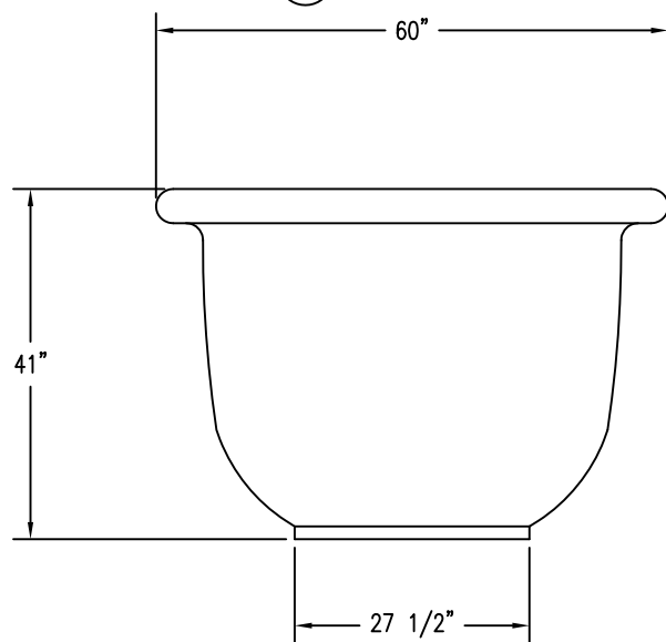
2 ELEVATION VIEW
