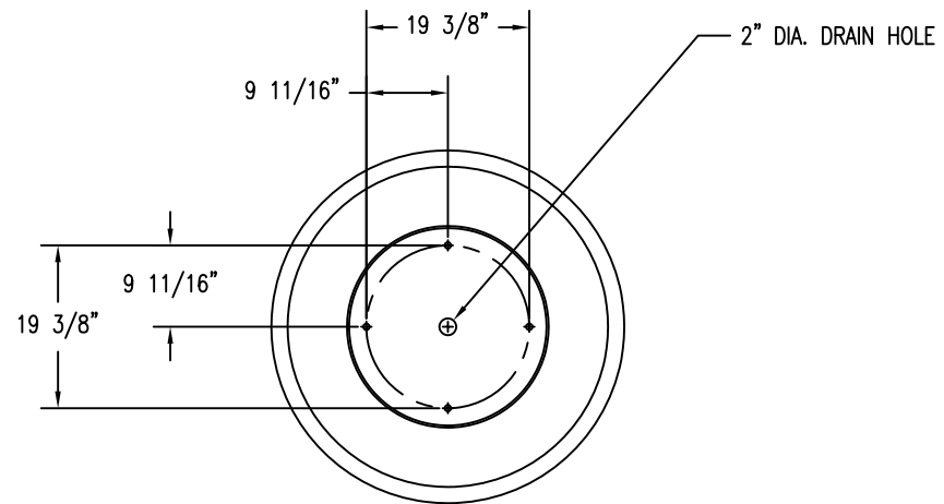
3 BOTTOM VIEW
