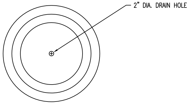
1 TOP VIEW
