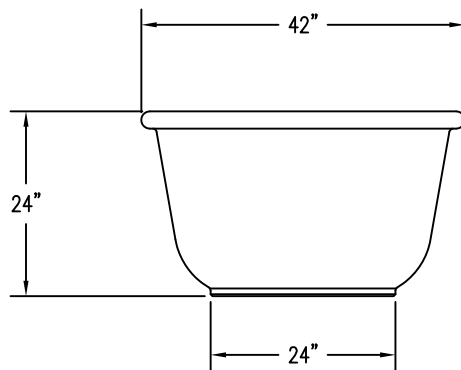
2 ELEVATION VIEW
