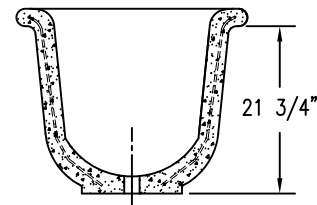
4 CROSS SECTION
