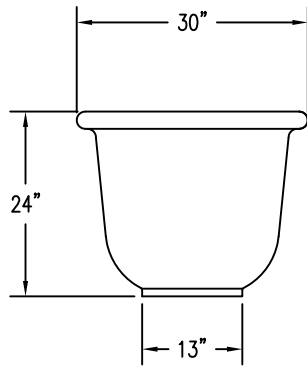
2 ELEVATION VIEW
