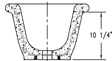
4 CROSS SECTION
