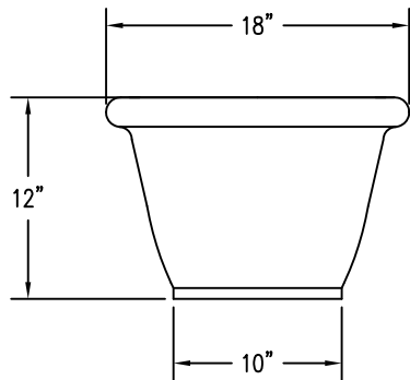
2 ELEVATION VIEW
