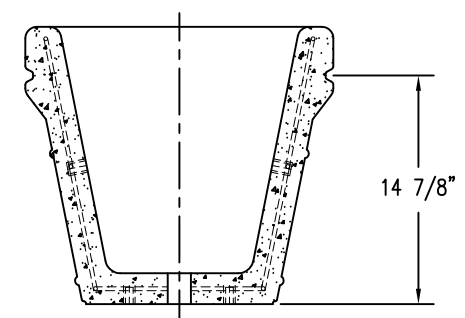
4 CROSS SECTION
