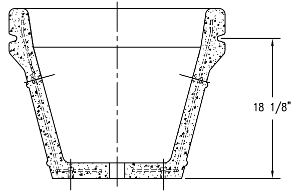
4 CROSS SECTION
